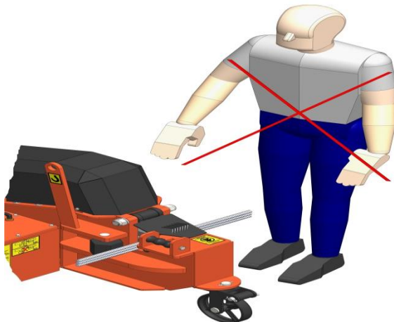
Figure 2(a,b): Wrong placement of the irons on the machine
